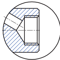
Screwed End Connection
